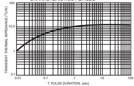
FIG.6- TYPICAL TRANSIENT THERMAL CHARACTERISTICS PER LEG
